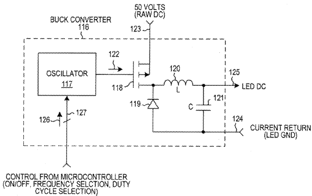
BUCK CONVERTER
